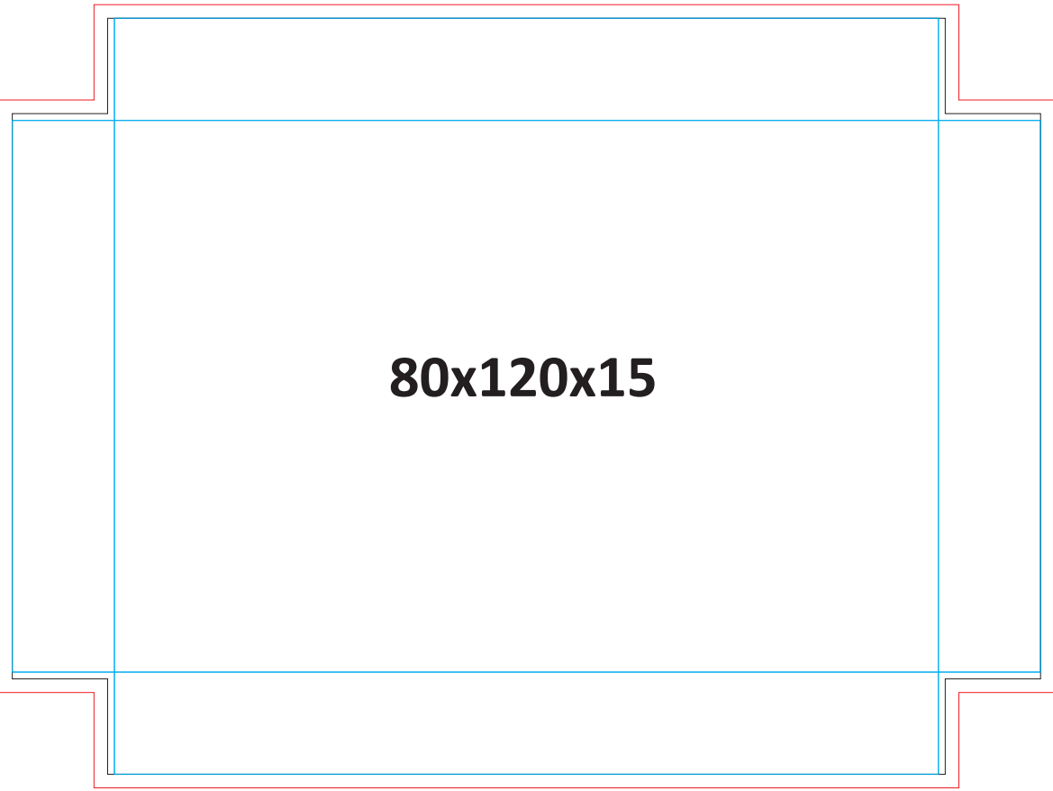
Pallet Covers (decotex205) sides sewing, bottom cut
